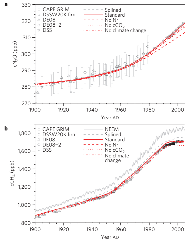
Figure 2 | Simulated and observed concentrations. a, b. Observed and simulated cN 2 O (a) and cCH 4 (b). Observational N 2 O data (grey) is from refs 22,33. Measurement precision ( \pm 1\sigma ) is given by vertical bars. The dashed grey line is a 200-yr cutoff spline through observational data. Observational CH 4 point data (grey) are from ref. 22 and represent Southern Hemispheric concentrations. The solid grey line (NEEM) is derived from Northern Hemispheric firm air data and includes seasonal variability 34 . The dashed grey line is a spline of observational Southern Hemisphere data. Simulation results (red) are from offline experiments where changes in climate, cCO 2 and Nr inputs are prescribed (standard), or where climate is held at pre-industrial levels (no climate change), cCO 2 is held constant at pre-industrial levels (no cCO 2 ) or Nr is held at pre-industrial levels (no Nr, see Supplementary Table S2). An oceanic N 2 O source (3.3 Tg N 2 O – N yr -1 ) and a constant geological CH 4 source (38 Tg CH 4 yr -1 ), tuned to match RCP data in year AD 1900, are included.
