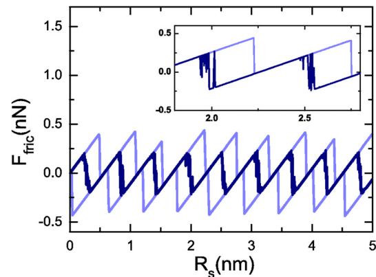
FIG. 4. Simulated friction force loops with (dark blue) and without (light blue) superimposed lateral oscillations. Parameter values: a = 0.564\text{ nm} , U_0 = 0.38\text{ eV} , k = 0.95\text{ N/m} , A = 0.6a , f = 180.3\text{ kHz} , v_s = 10\text{ nm/s} , and T = 300\text{ K} . The inset shows the back-and-forth jumps accompanying the transition from a lattice site to the next one. As in Fig. 2, the lateral force is averaged over 180 (36 in the inset) oscillation cycles.
